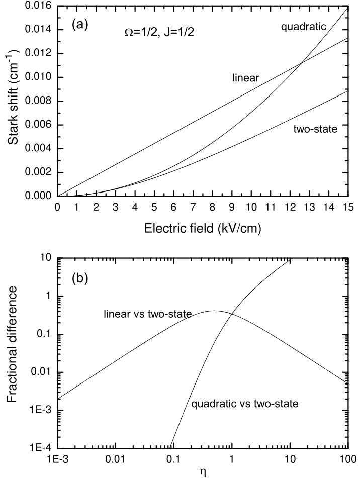
FIG. 2: (a) The dc Stark shifts for the v = 0 , J = 1/2 state of the {}^2\Pi_{1/2} spin-orbit level as a function of electric field strength. Shifts in the two-state model and in first- and second-order perturbation theory are shown over an experimentally realistic range of field strengths. (b) The fractional difference between Stark shifts, as calculated using perturbation theory and using the two-state model [see Eqs. (20)], for a rovibronic state of a Hund’s case (a) molecule. First- and second-order perturbation theory give the linear and quadratic approximations, respectively. The parameter \eta , the Stark matrix element normalized to the \Lambda -doublet splitting, is defined in Eq. (19).
